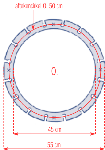
1. zaagplan ringen
