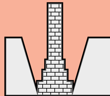
gemetselde fundering
