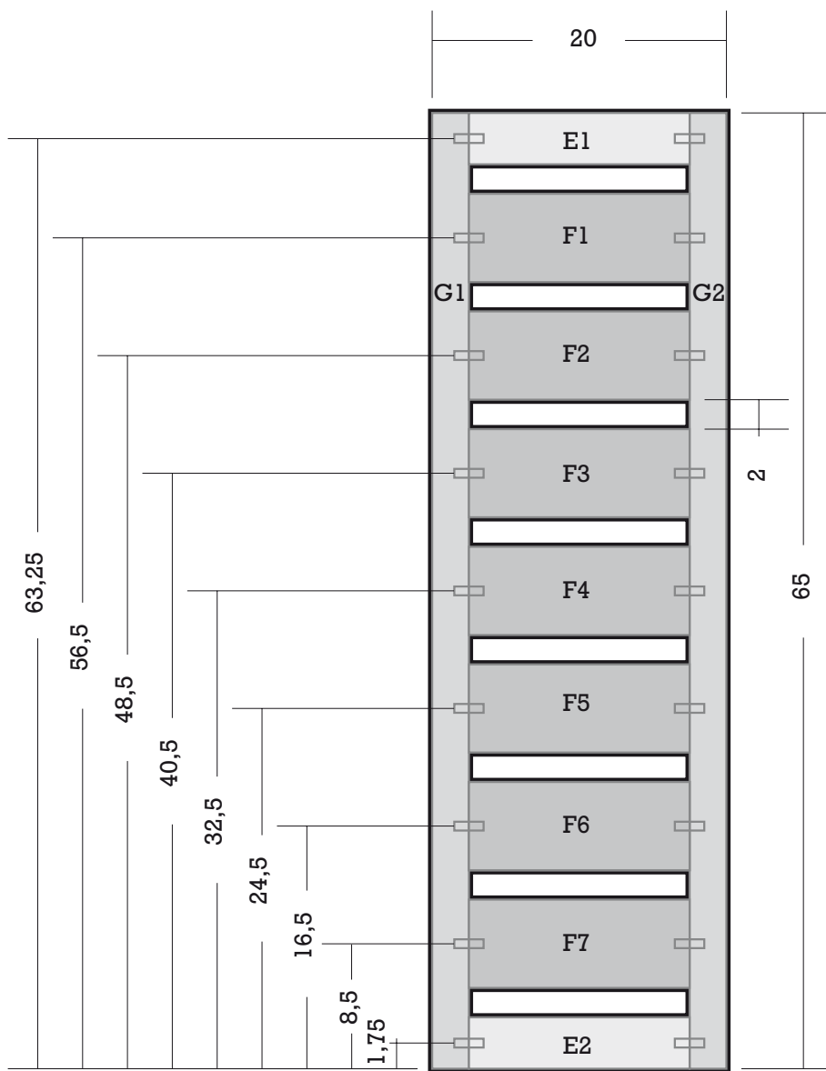
Tekening 1 (A1) (maten in cm)
